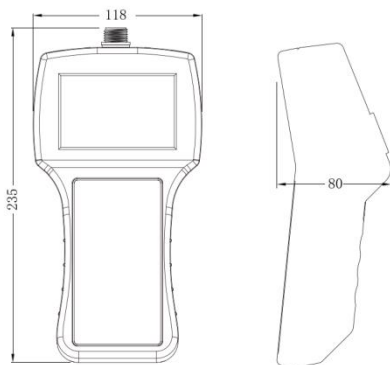
Appearance size diagram
