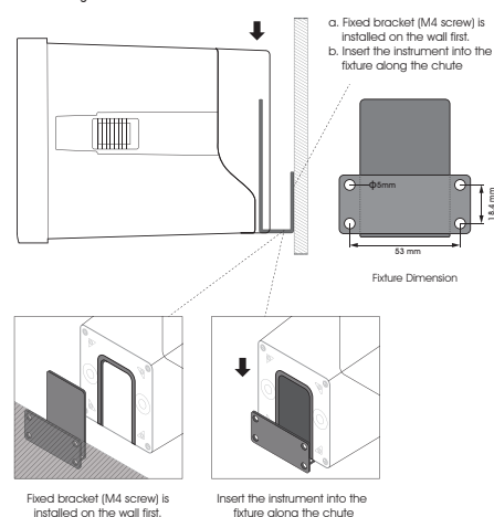
Wall mounting
