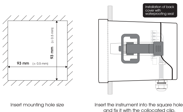
Embedded installation
