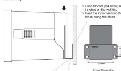
Wall mounting
